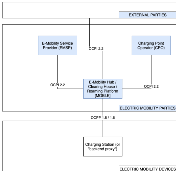
Figure 4 Reference Architecture for Phase 2
